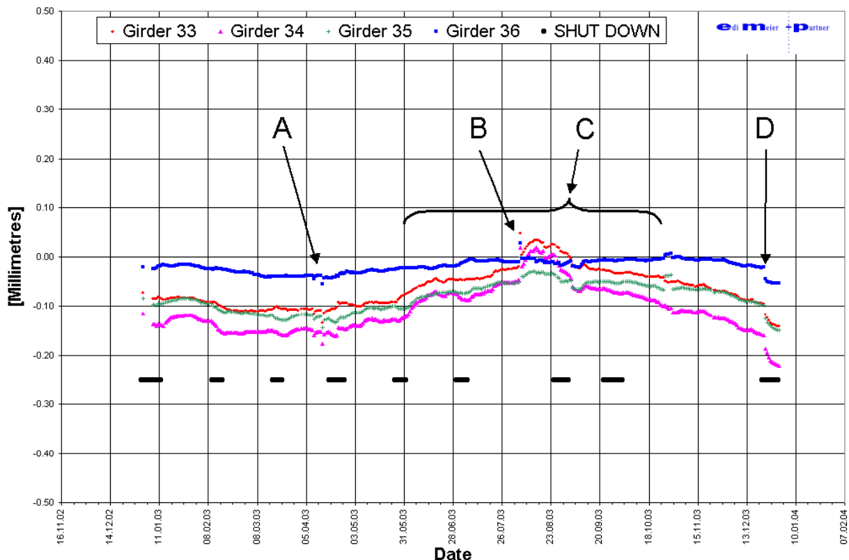
Fig. 9: Long-term monitoring in sector 9 (4 girders) of the PSI-SLS. Clearly visible are a system purging (A) and filling (B). The exceptional hot summer of 2003 made it necessary to raise the operating temperature by several degrees. While the girders 33 – 35 show a significant reaction to this change in temperature (C), girder no. 36 stays almost steady. The reason are the cooling pipes for the SLS which are located near that girder, causing a lower temperature at this particular spot. During the shutdown in December 2003 (D) several heavy shielding elements have been placed temporary on the roof of sector 9. That event caused vertical displacements in this sector.
