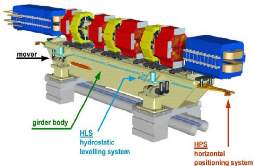
Fig. 4: Girder body carrying the electromagnets. The movers are intended to move the whole girder in order to re-adjust the electromagnets. The girder movement is monitored by the HLS.
