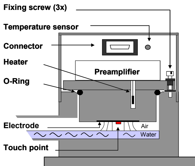
Fig. 2: Cross section of a HLS level sensor.
