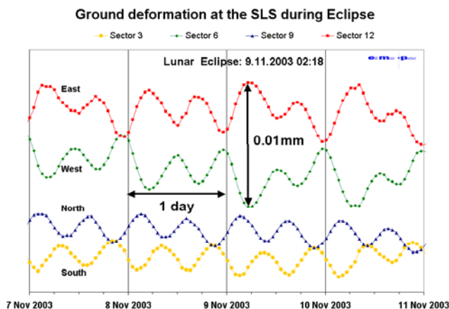
Figure10: A four day period of the year 2003 with a time resolution of 1 hour. The influence of the earth tides with 2 periods a day is clearly visible. Note the high amplitude difference between east and west during the eclipse of the moon.
