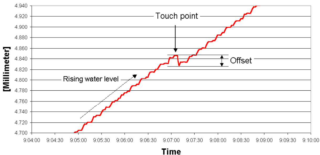
Fig. 3: Detection of the touch point during the filling process. For every level sensor this point is well defined. The slope of the signal is constant. After the touch point has been reached, a constant offset from the true level signal is subtracted. In this way, by the use of just one data channel the following information can be retrieved: “the current fluid level” and “the touch point has been reached”.
